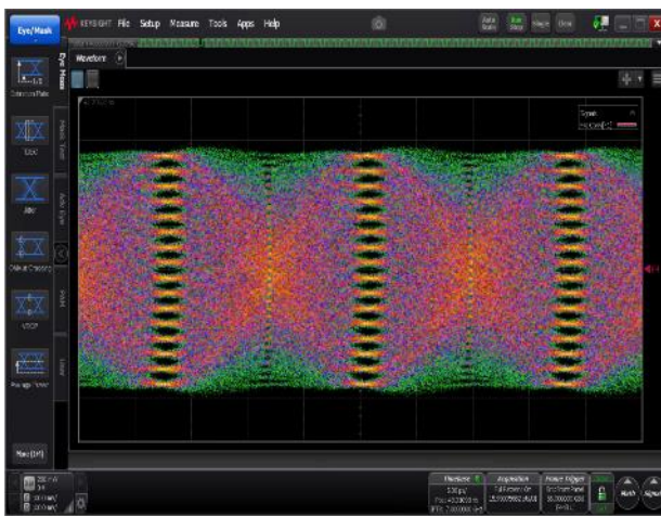
Figure 2. 56 GBaud PAM16 (= 224 Gbps)
